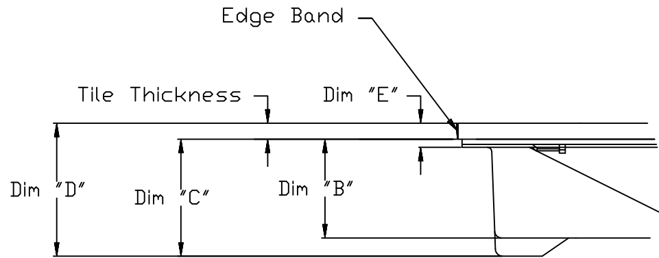
DETAIL A SCALE 1 : 4
