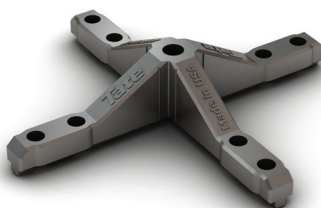
Perimeter Connector
