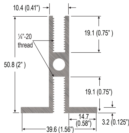
1/4"-20 Slot
